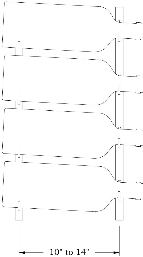
(Standard Mounting) Front View
